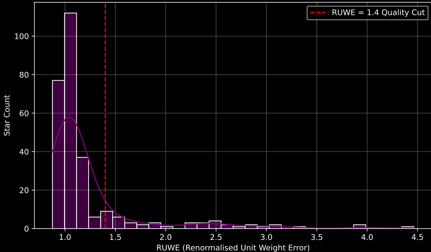
GALAH DR4 Field [190] RUWE Distribution (n= 278)
