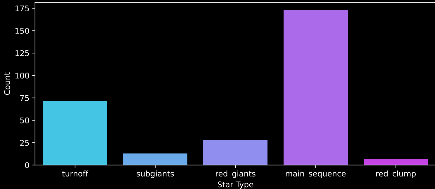
GALAH DR4 Field: [190] Count plot of Star Type
